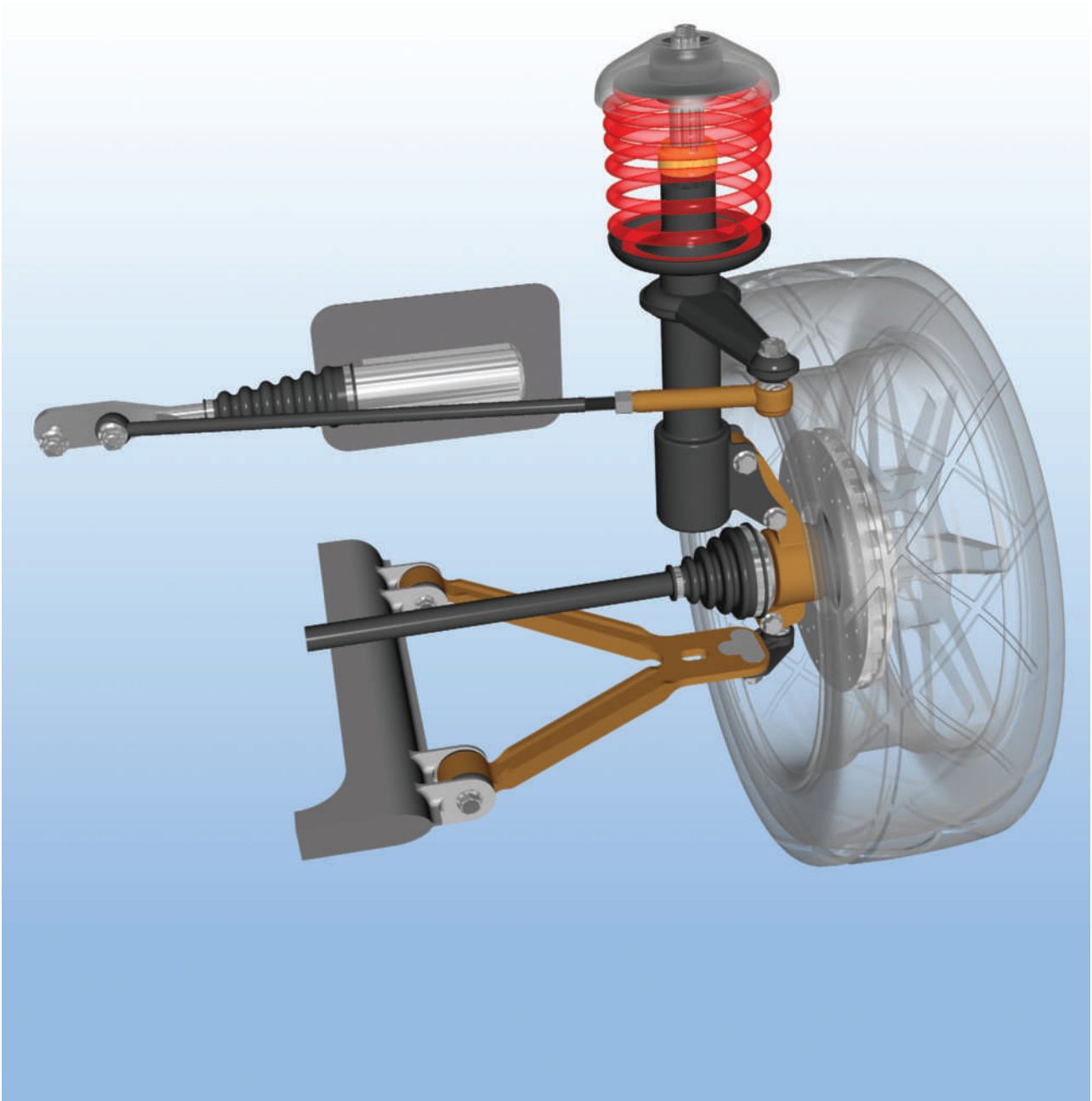
This illustration shows the elements of the left-front suspension on an all-wheel-drive automobile. The spring and shock absorber are coaxial in this McPherson-strut type of suspension.
