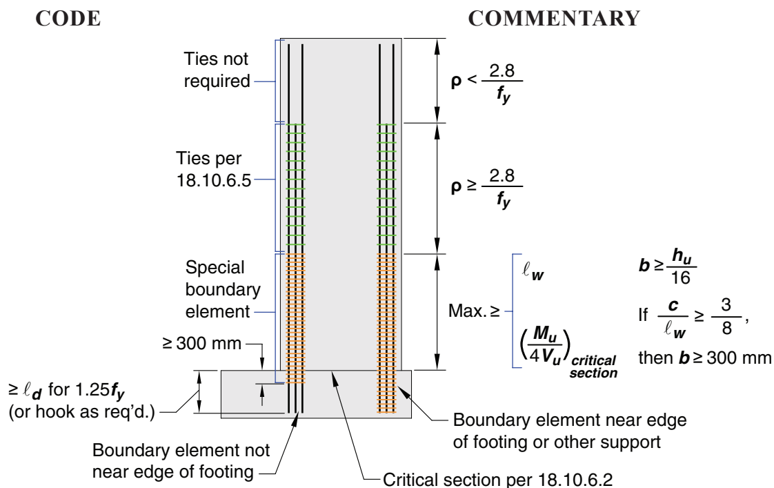
(a) Wall with h_w/\ell_w \geq 2.0 and a single critical section controlled by flexure and axial load designed using 18.10.6.2, 18.10.6.4, and 18.10.6.5
