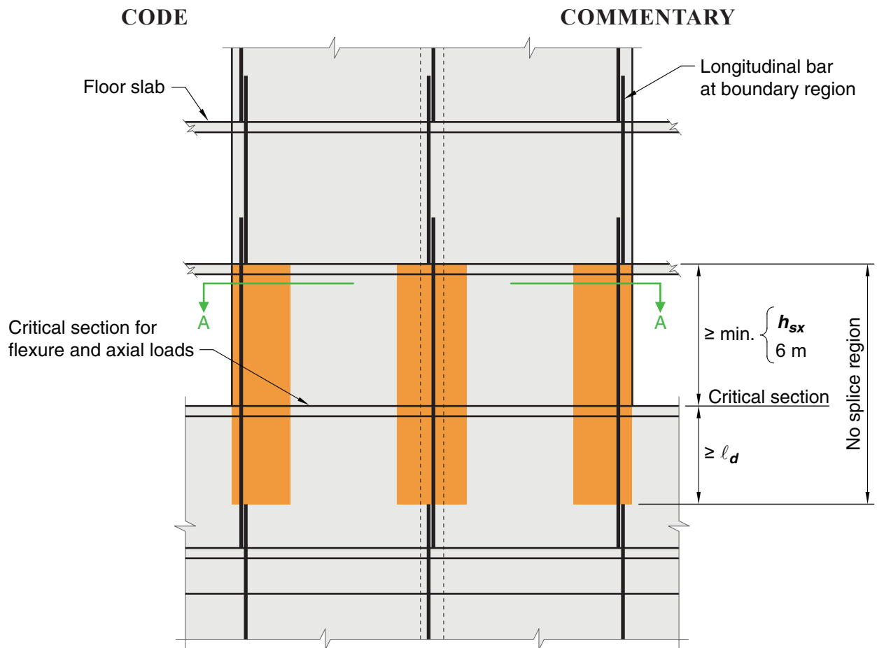
(a) Elevation
