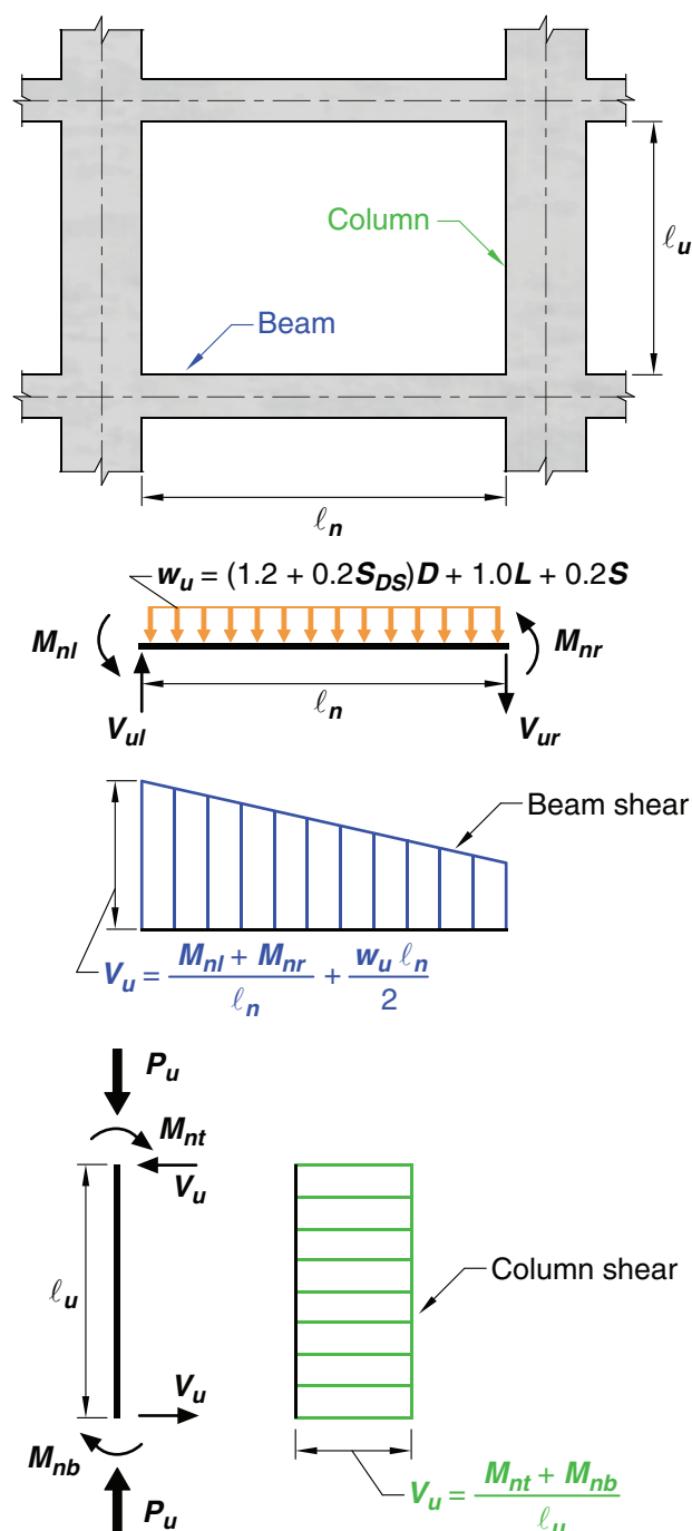
Fig. R18.4.2 —Design shears for intermediate moment frames.
