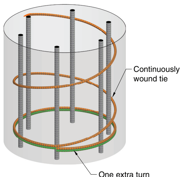
Fig. R25.7.2.3b —Continuous tie anchorage.
