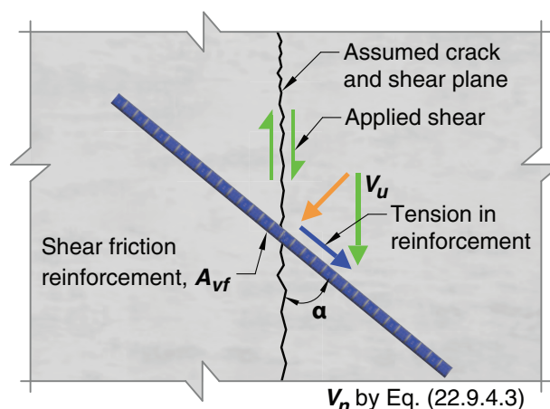
Fig. R22.9.4.3a—Tension in shear friction reinforcement.
