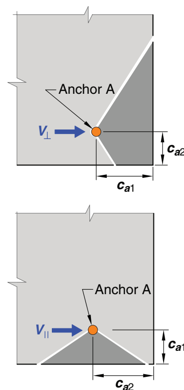
Fig. R17.7.2.1d—Shear near a corner.
