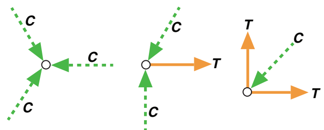
Fig. R23.2.6c —Classification of nodes.
