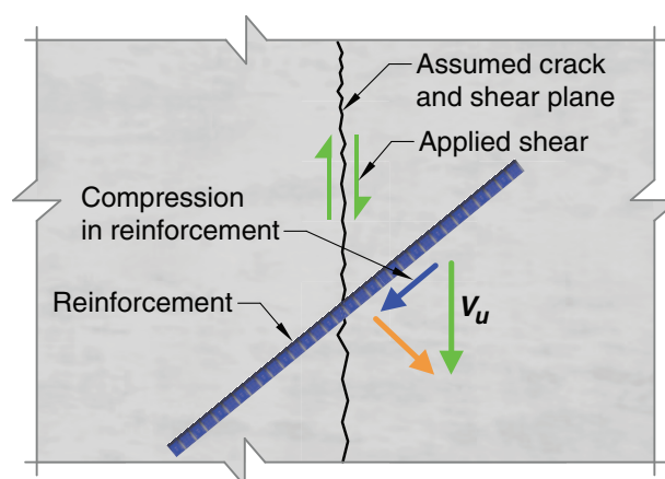
Fig. R22.9.4.3b—Compression in reinforcement.
