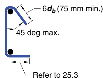
(a) single-leg stirrup or bar
